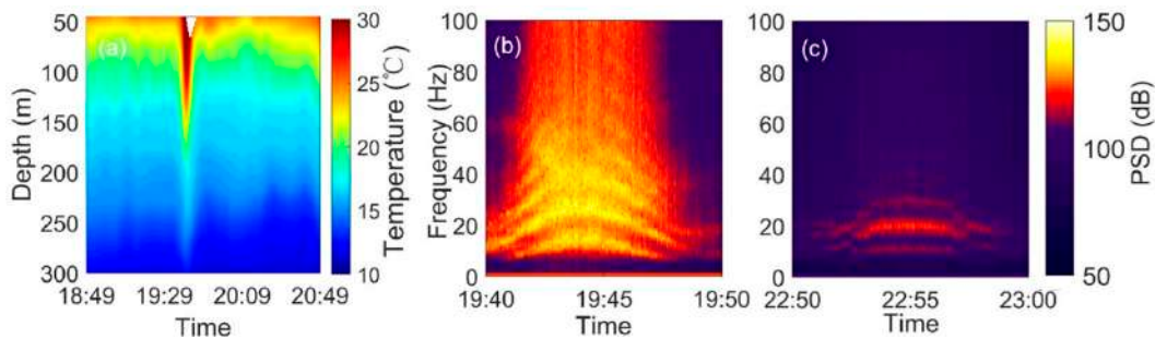
Figure 8. Temperature data and noise of the same ISW received by two hydrophones on 9 July 2019. (a) Temperature measured by the thermistor chains. (b) Time–frequency spectrum from a hydrophone at a depth of 250 m. The cable of the hydrophone array is 300 m long. (c) Time–frequency spectrum from the near–bottom hydrophone at a depth of 340 m. The cable of the single hydrophone is 30 m long.
