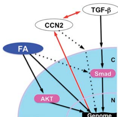
Figure 8. Possible cartilage regeneration mechanism by FA in collaboration with TGF- \beta . N, Nucleus; C, cytoplasm; FA, fluocinolone acetonide.
