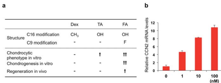
Figure 7. (a) Structural–functional relationship of three glucocorticoids. TA, triamcinolone acetonide; FA, fluocinolone acetonide. (b) Induction of CCN2 in ATDC5 chondrogenic cells by FA. ATDC5 cells in monolayer culture were treated with different concentrations (1–100 nM; horizontal axis) of FA for 24 h, and analyzed for expression levels of CCN2 mRNA.
