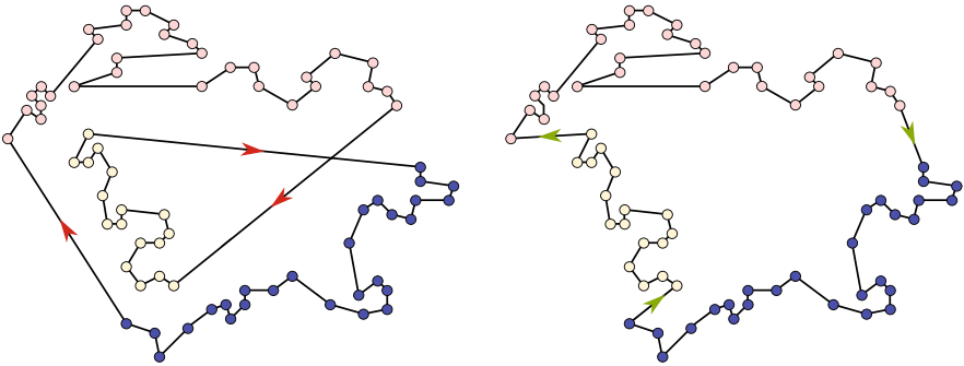
Fig. 5.4 3-opt move. Three arcs are replaced by three others. They connect three sub-paths traversed in the same direction, before and after modification. Another way to apprehend the 3-opt neighborhood is the displacement of a sub-path elsewhere in the tour
