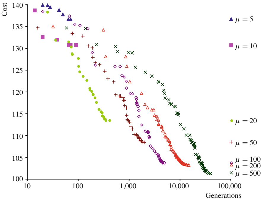
Fig. 10.10 Influence of the population size on the solution quality. When the population is too limited, it converges very rapidly with a low probability of discovering good solutions. Conversely, a large population converges very gradually, but better solutions are obtained
