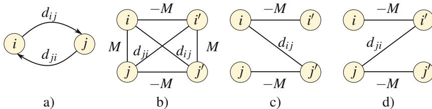
Fig. 1 Principle of a polynomial transformation of an asymmetric traveling salesman problem into a symmetric one. (a) Two nodes i and j of the original directed graph. (b) Doubling of nodes and weights in an undirected graph; M is a sufficiently large constant value. (c) A possibility of visiting vertices i and j in the undirected graph, without having to pay the M penalty and by collecting a bonus of 2M , corresponding to a visit in the order i \rightarrow j in the directed graph. (d) The only other reasonable possibility, corresponding to a visit in the order j \rightarrow i
