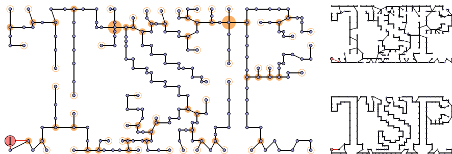
Fig. 3.6 Left: 1-tree on the TSP instance tsp225 obtained with all \lambda values set to 0. The size of filled disks is proportional to the value to add to the \lambda associated with penalized vertices, and circles are proportional to the value to remove. Top right: the 1-tree obtained with the first modification of the \lambda . Bottom right: the 1-tree obtained after iterating the process. Only 12 vertices have a degree different from 2, and the length of this 1-tree is about 7.5% above the length of the initial 1-tree and 1.1% below the optimum tour length
