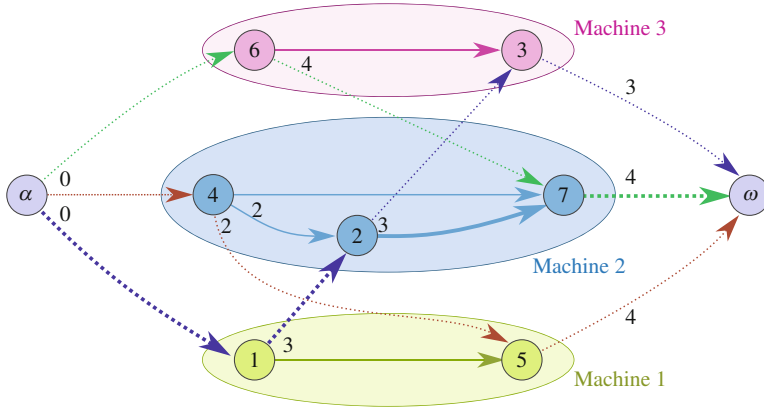
Fig. 2.5 Graph corresponding to the solution of a jobshop instance with three machines. One job undergoes 3 operations while two others have only 2. The weighting of the arcs corresponds to the duration of the corresponding operation. The arcs representing the precedence relations of the operations belonging to the same job are in dotted lines. The longest path from \alpha to \omega is shown in bold. It is referred to as the critical path
