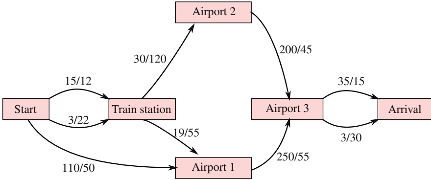
Fig. 3.7 Example of a multi-objective problem: To travel from a departure place to a destination, several routes can be selected. Each trip has a given cost and duration, indicated next to the arcs. From the departure place, we can either go to the train station by bus, or by taxi, or go directly to the nearest airport by taxi. From the train station, we can reach either the nearest airport or another airport. The last is a little further away but better serviced and flights are more competitive. Then we fly up to the airport the closest to the destination, where we can go to the final destination either by bus or by taxi
