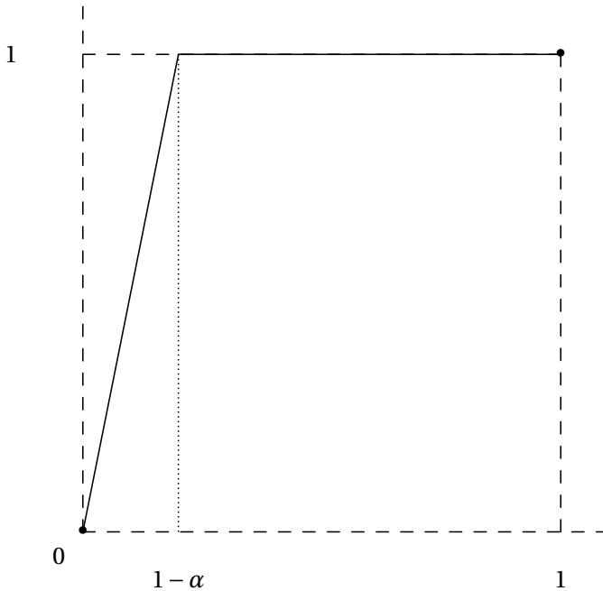
Figure 5.3 Distortion function of the \text{TVaR}_\alpha risk measure
