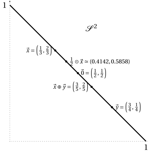
Figure 8.1 Example of perturbation (addition) and powering (scalar multiplication) in \mathcal{S}^2
