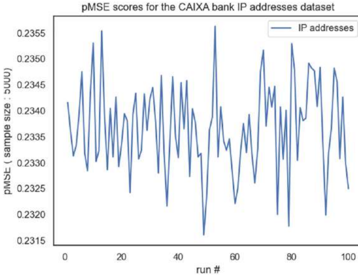
Fig. 4 Results for 100 random sampling taken from the real and synthetic data (5 K datapoints each) and the pMSE calculated using a logistic model
