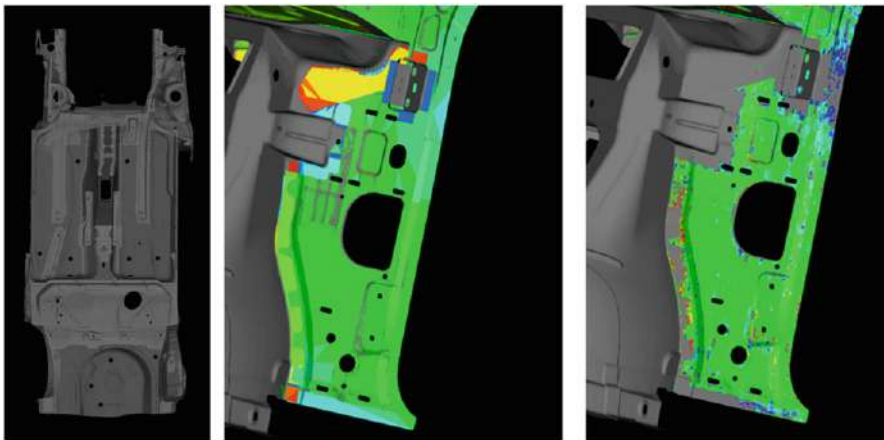
Fig. 19 Large-scale CAD file (left), annotated polygonal colormap mesh (middle), textured colormap mesh (right)
