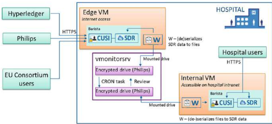
Fig. 4 Software architecture
