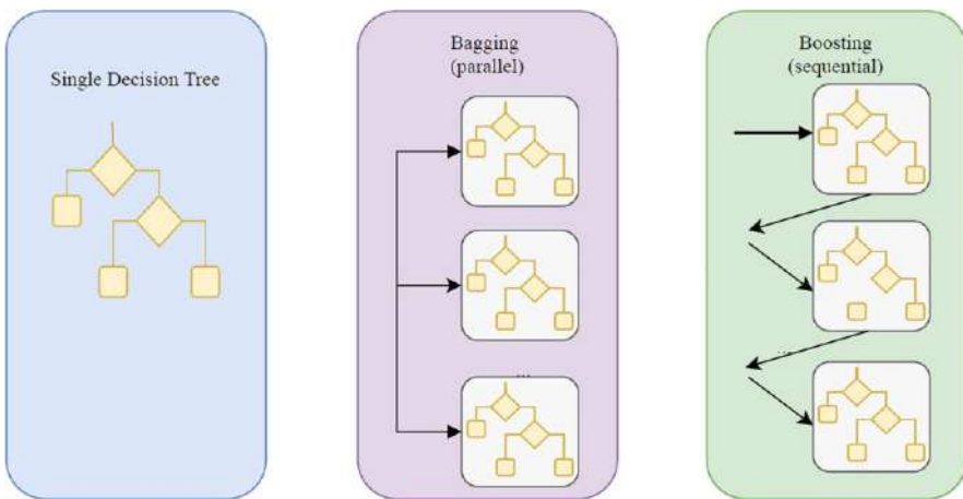
Fig. 2 Decision trees and ensemble methods
