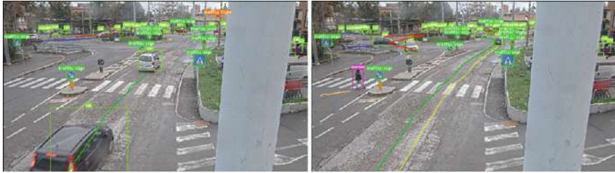
Fig. 4 Object tracking output from street camera detections
