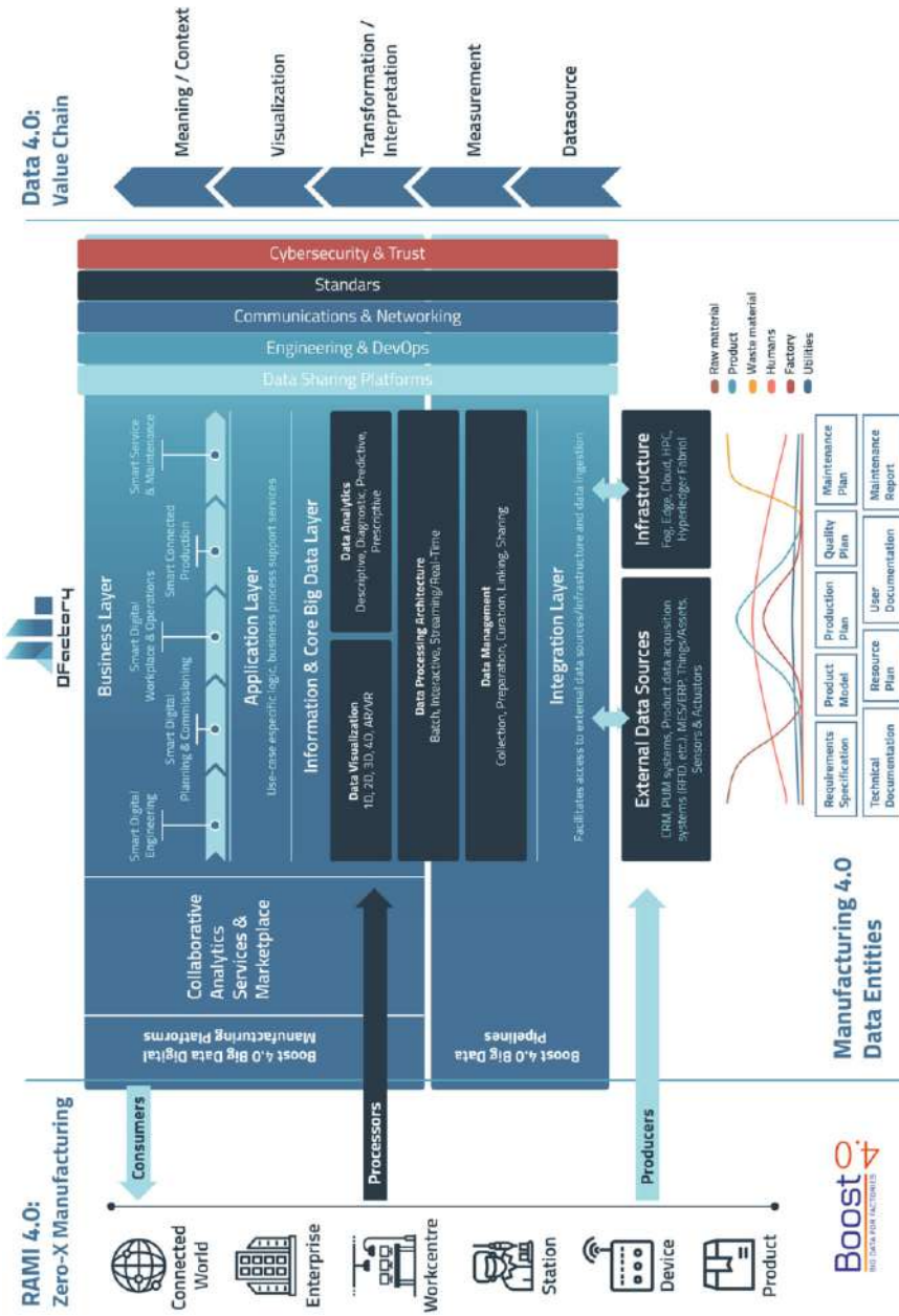
Fig. 2 Boost 4.0 Universal Big Data Reference Architecture 4.0
