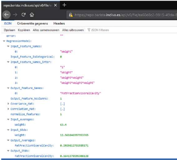
Fig. 13 The polynomial regression model
