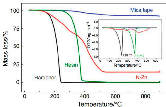
Figure 26. TG/DTG curves of components obtained under N 2 atmosphere (10 °C·min -1 ), PT pan, and β of 10 °C·min -1 . © copyright permission Springer, 2011, Journal of Thermal Analysis and Calorimetry, Thermal characterization of mica–epoxy composite used as insulation material for high voltage, License No. 3837180507265 [83].
