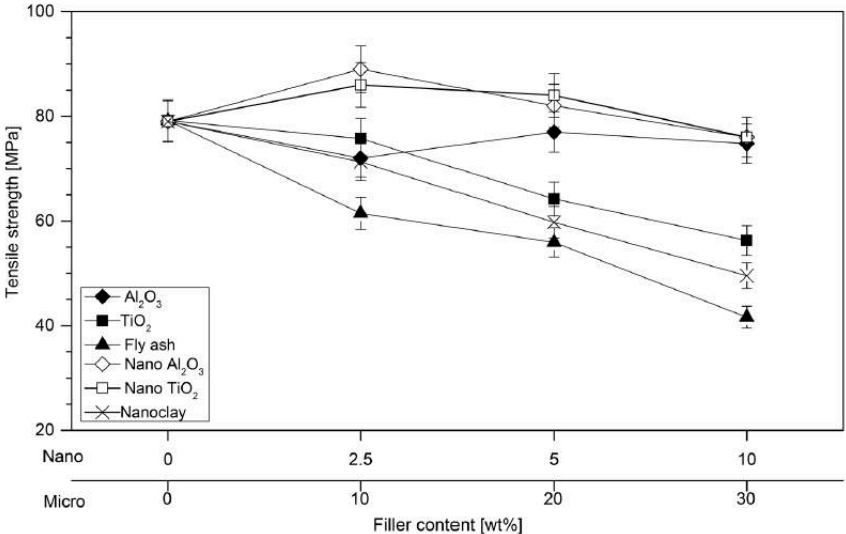
Figure 42. Tensile strength of epoxy resin based micro/nanocomposites versus filler content (Reprint with the permission of Strojniski vestnik–Journal of Mechanical Engineering [191]).
