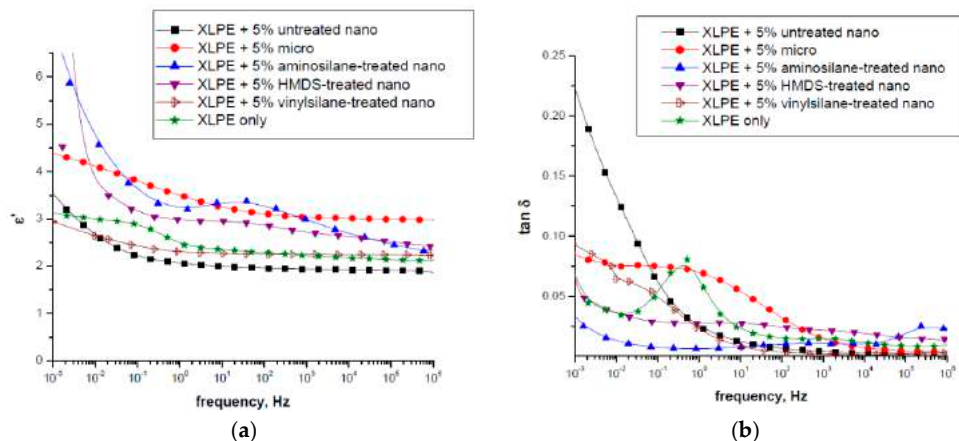
Figure 25. (a) Real part of relative permittivity and (b) loss tangent of functionalized XLPE at 23 °C (© 2016 IEEE. Reprinted, with permission, from [102]).
