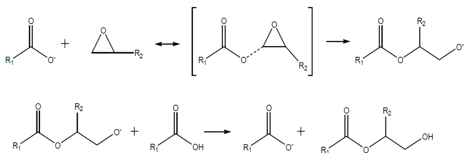
Figure 15. Carboxylate-epoxy reaction.
