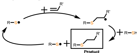
Scheme 2. Schematic representations of the decomposition of the photoinitiator ( top ) and the thiyl-thiyl cycle of the thiol-ene reaction ( bottom ).
