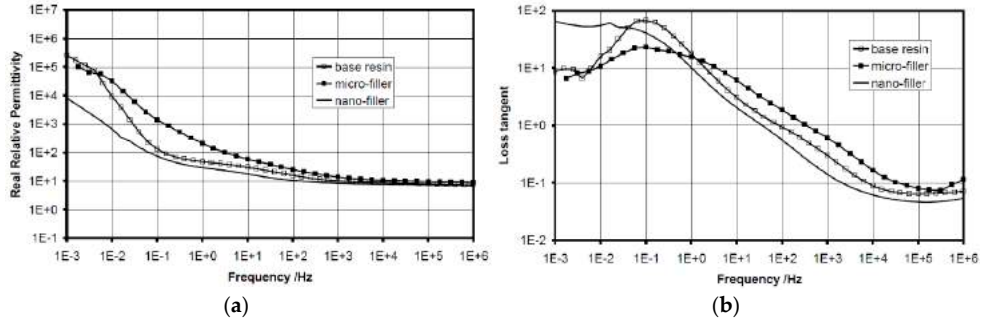
Figure 24. (a) Real part of relative permittivity and (b) loss tangent of unfilled epoxy resin and epoxy/ 10 wt % TiO 2 micro/nanocomposites materials at 393 K (© IOP Publishing. Reproduced with permission. All rights reserved [22]).
