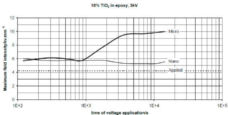
Figure 30. Maximum field intensity as a function of voltage time application on epoxy/ \text{TiO}_2 micro/nanocomposites (© IOP Publishing. Reproduced with permission. All rights reserved [22]).
